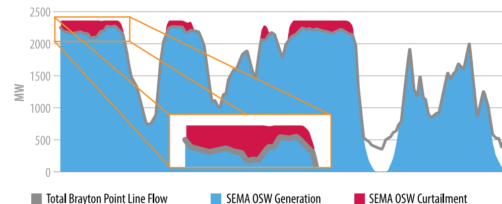
Base Case SEMA Offshore Wind Generation and Curtailment at Brayton Point (One Week)
